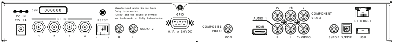
Figure 1: Unity 552 rear panel view with HDMI port
